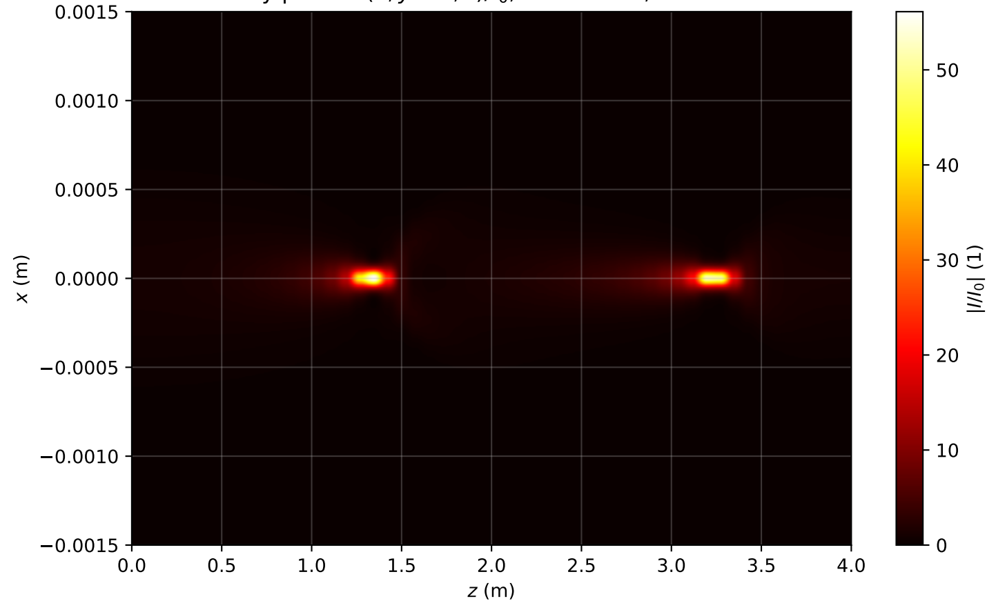
Intensity profile I(x, y = 0, z)/I_0 , P_{in}=1.8P_{cr} , artificial time
